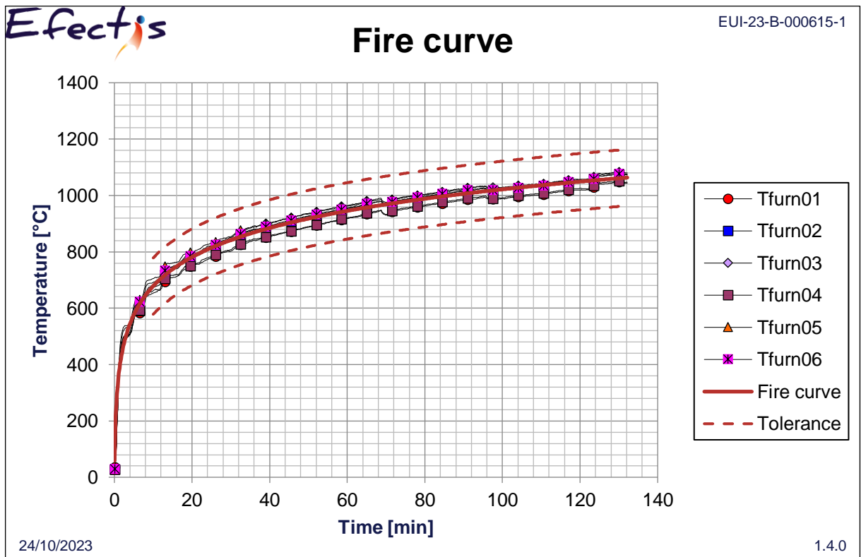
Chart 2 - Furnace temperature during the test
