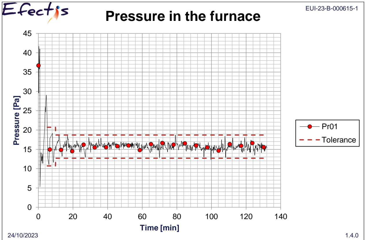
Chart 4 - Furnace pressure during the test
