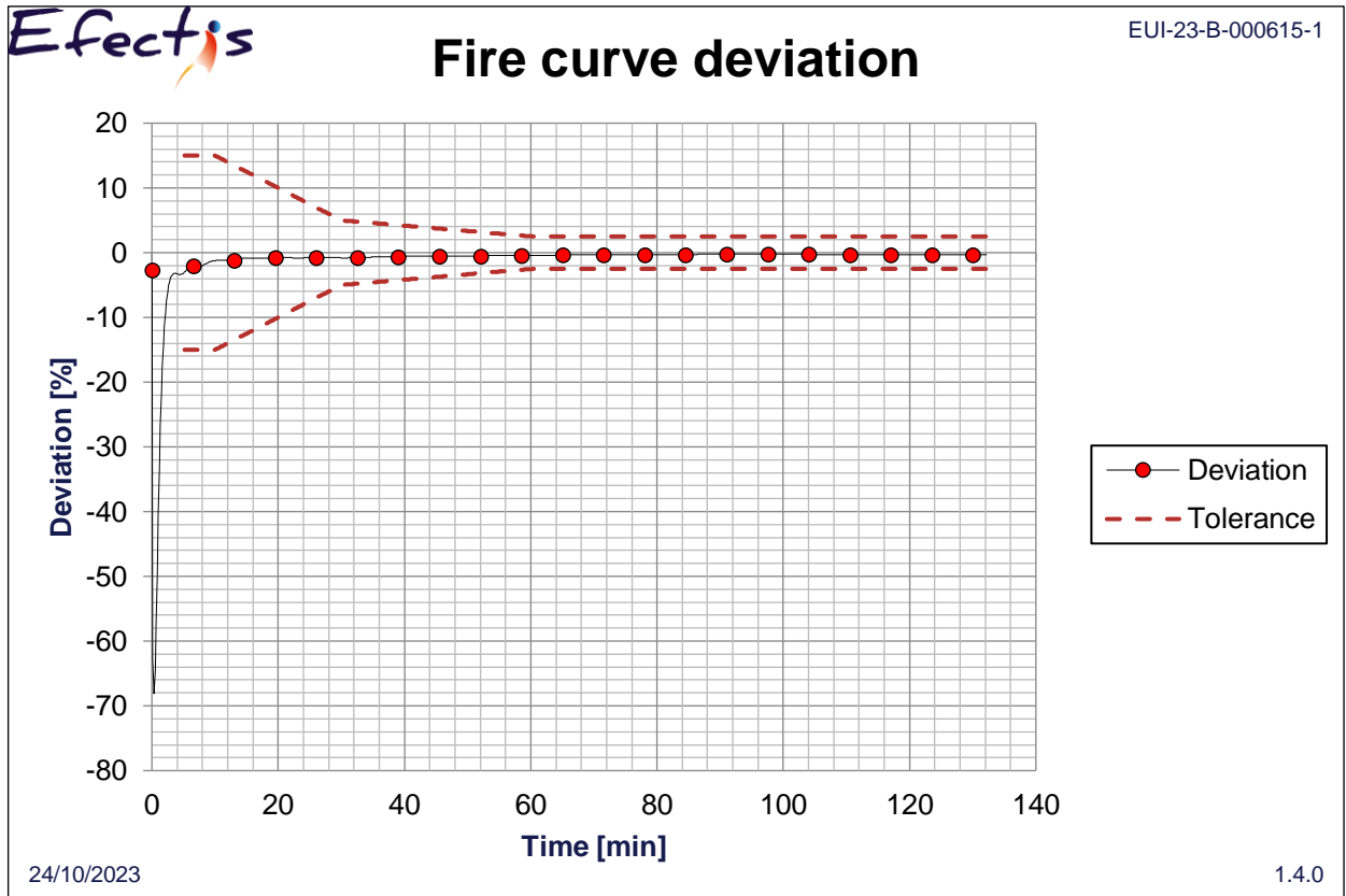
Chart 3 - Deviation curve of fire during test
