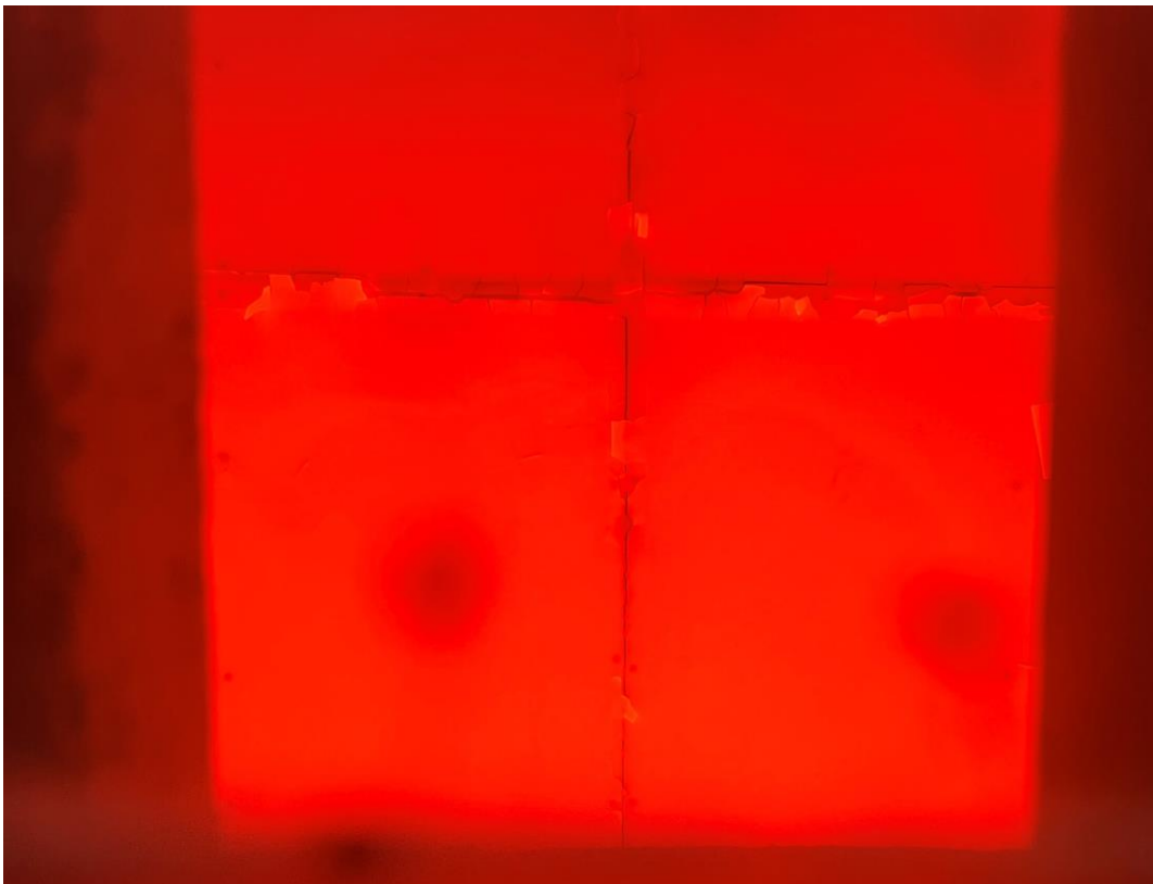
Photo 8 - Exposed side of the specimen - Min 38
