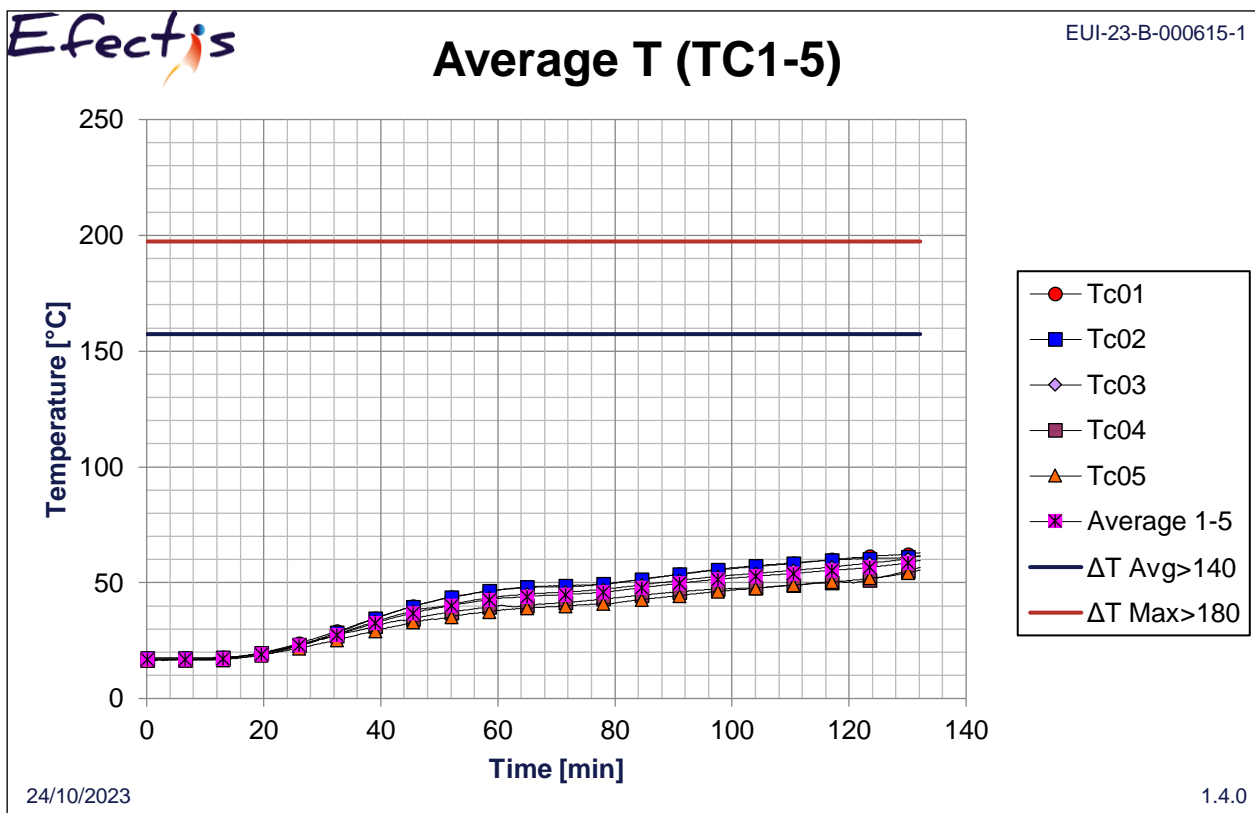
Chart 5 - Average temperature of unexposed side during the test
