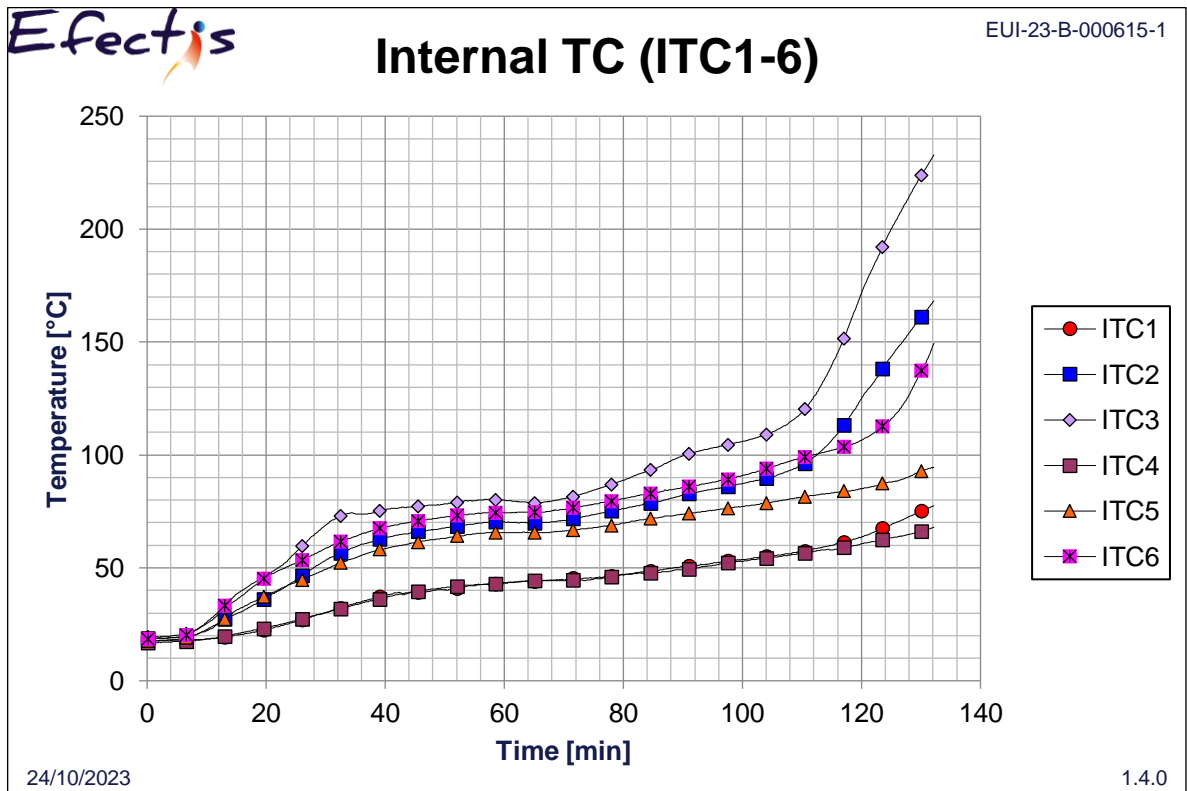
Chart 8 - Plot of internal thermocouples
