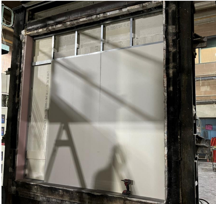
Photo 3 - Specimen during construction - Exposed side boarding – first layer. Note the boards over the angles on the horizontal joints.
