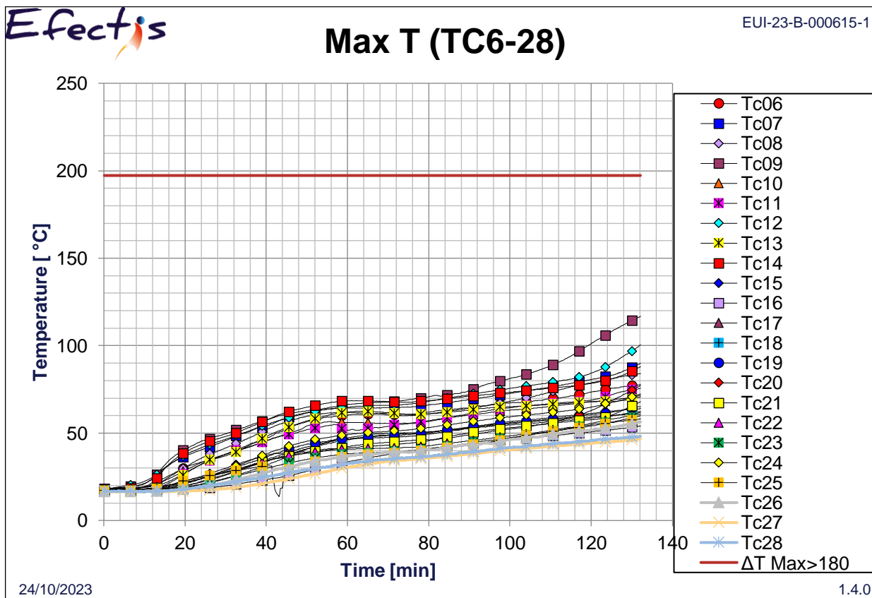
Chart 6 - Maximum temperature during the test
