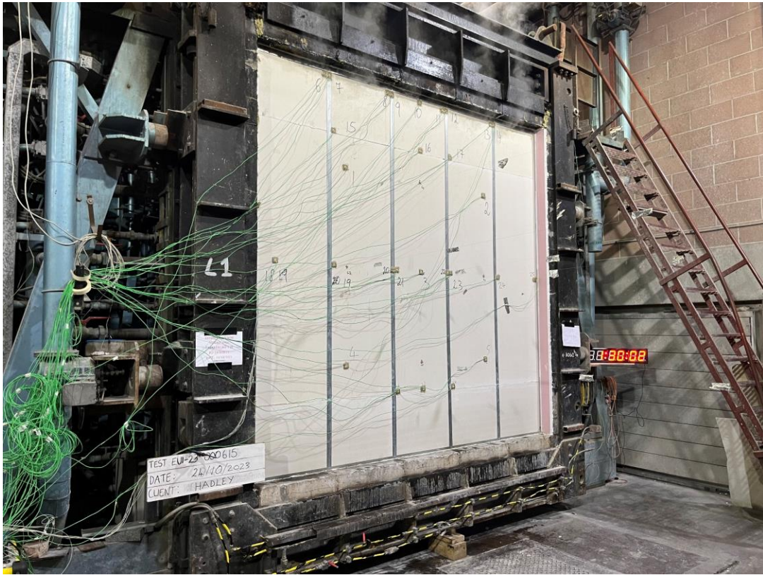
Photo 9 - Unexposed side of the specimen - Min 90
