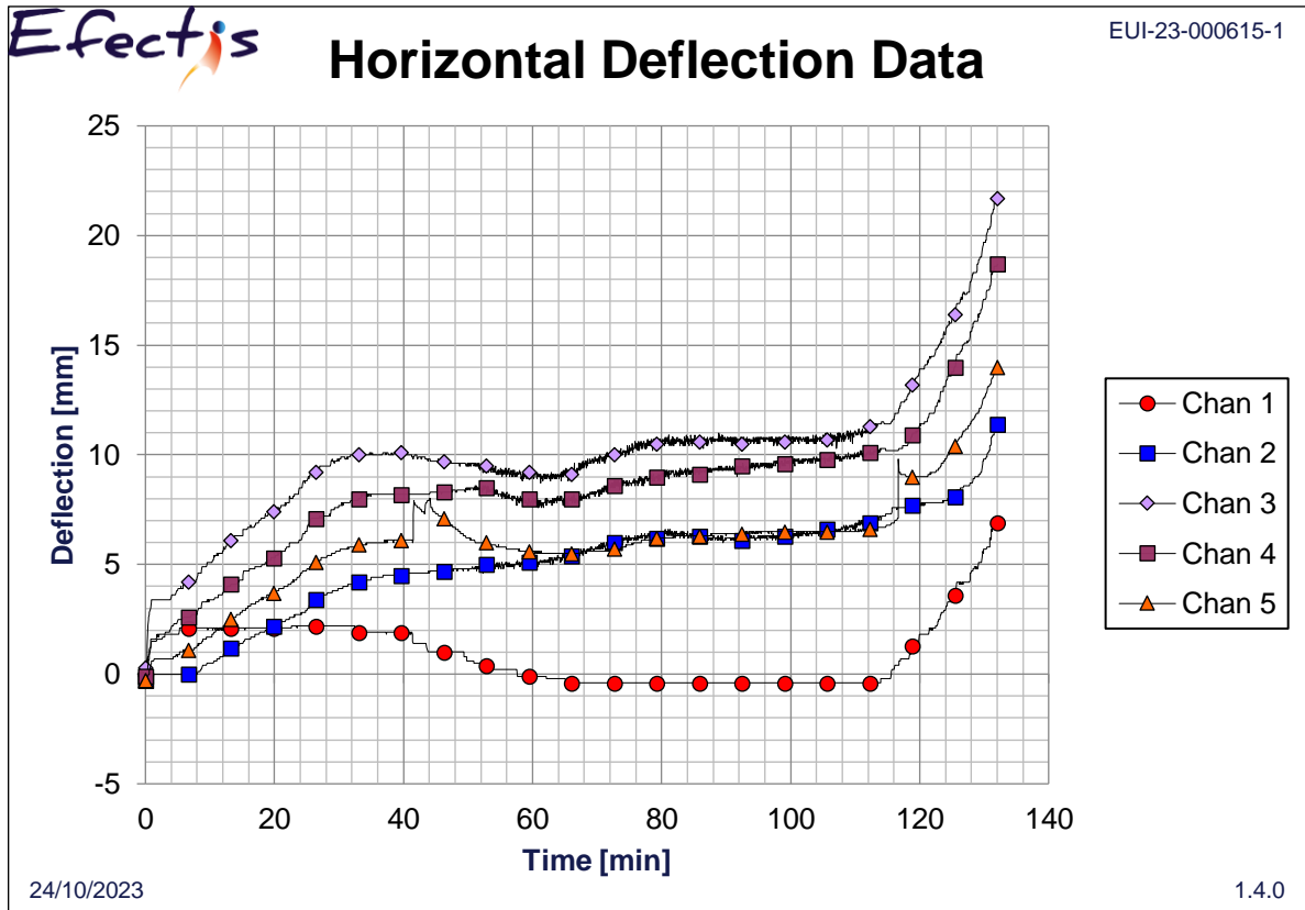
Chart 7 - Horizontal deflection during the test
